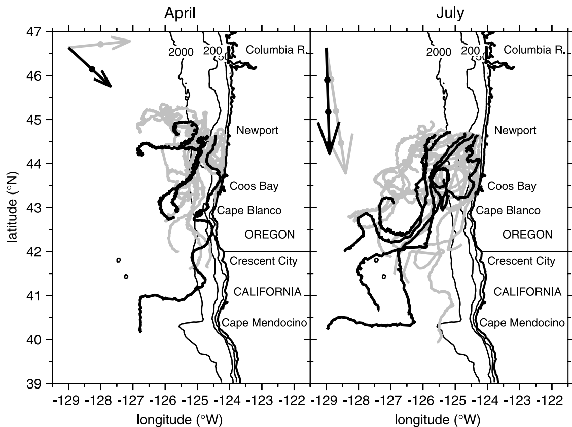
Figure 1. Drifter trajectories over 30 days originating from five cross-shelf locations from deployments in April (left) and July (right). Trajectories from 1998–2001 are in gray and those from 2002 are black. Average wind stress vectors over 30 days from NOAA NDBC buoy 46050 37 km offshore of Newport for 1998–2001 (gray) and 2002 (black) are shown in the upper left of each panel. Tics along the wind stress vectors are at 0.01 \text{ N m}^{-2} intervals. Isobaths in meters.
