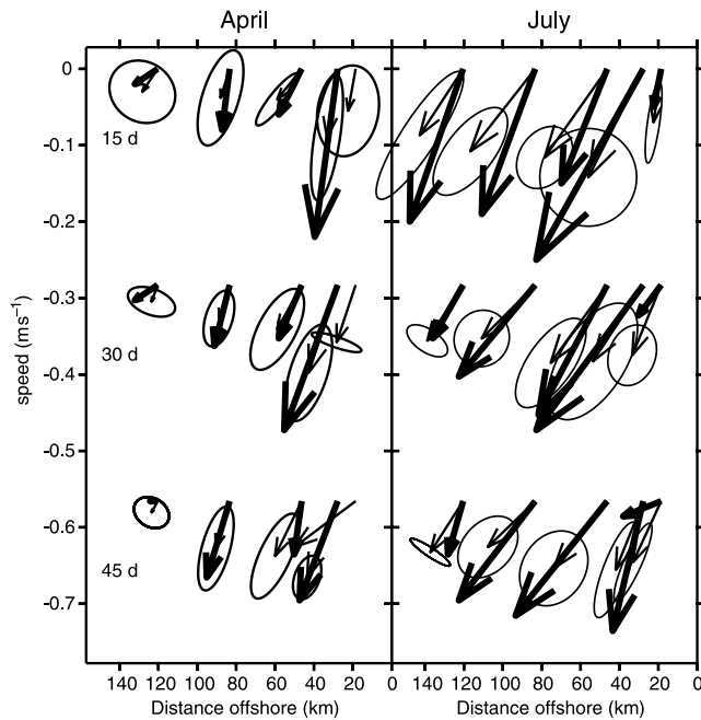
Figure 2. Drifter velocity vectors from five release locations across the shelf at 44.65^{\circ}\text{N} , averaged over 15, 30 and 45 d (top, middle, bottom) starting in April (left) and July (right). Thin vectors with standard deviation ellipses represent averages over all deployments from 1998 to 2002. Bold vectors are for 2002. Note that the most inshore drifter deployed in April 2002 grounded after just 9 days so no bold vector is plotted for that time and place. North is toward the top of the figure.
